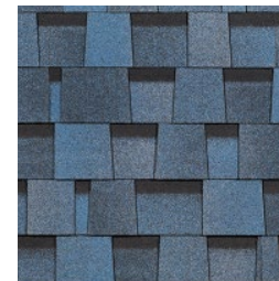
Sapphire
