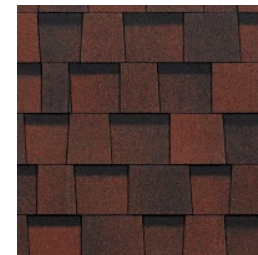
Jasper
