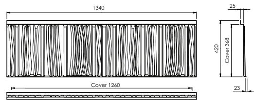
Tile Dimensions
