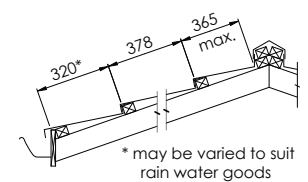
Batten Layout
